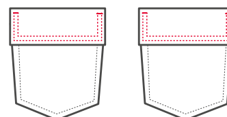
Top stitch for flap
